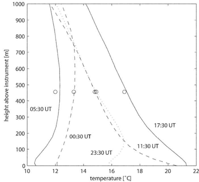
Figure 9 - Temperature profiles in the lowest km above ground at 5 different times on September 18, 2002 in Bern measured with ASMUWARA and comparison with data from a meteo station (circles) located on a nearby TV tower. After [58].
