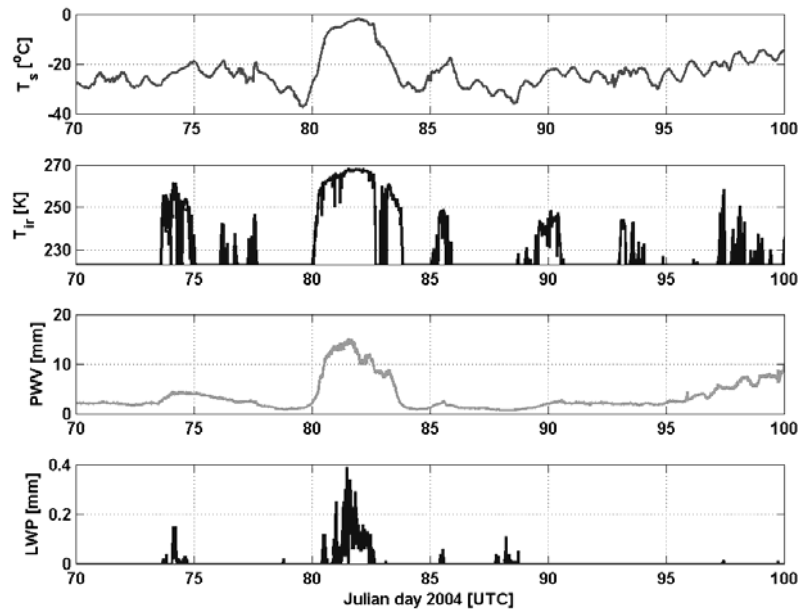
Figure 8 - Time series of surface temperature (top panel), infra-red measured cloud base temperature, 2 nd panel, PWV as measured by the MWRP, 3 rd panel, and LWP as measured by the MWRP, 4 th panel.
