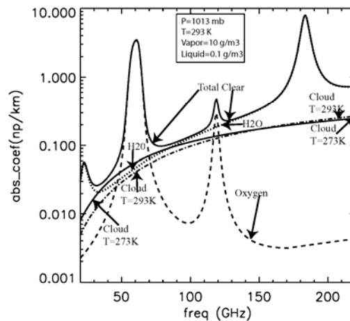
Figure 2 - Microwave absorption spectra from 20 to 220 GHz. The absorption models used were Liebe 89 [4] for clear absorption, and Liebe et al. 1991 [6] for cloud liquid. P = pressure, T = temperature, \rho_V = absolute humidity, and \rho_L = cloud liquid density.
