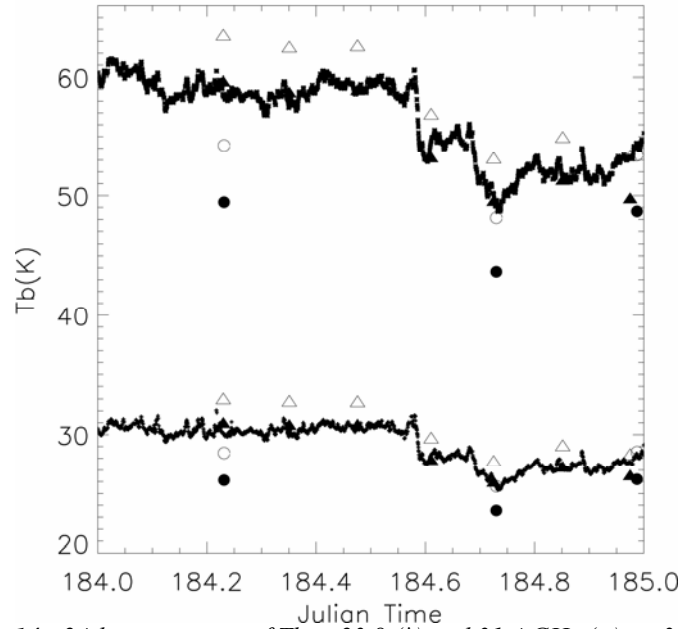
Figure 14 - 24-hr time series of T_b at 23.8 (*) and 31.4 GHz (+) on 3 July, 1999. Closed circles — calculated from original ARCS-2 radiosondes (age = 315 days). Open circles — calculated from corrected ARCS-2 radiosondes. Closed triangles — calculated from original RHB radiosondes (age = 172 days). Open triangles — calculated from corrected RHB radiosondes. RTE model [5]. After [62].
