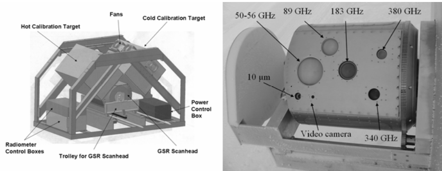
Figure 6 - Left. Schematic diagram of the GSR calibration and scanning system. The GSR scanhead periodically moves out of the framework for atmospheric viewing on a trolley system, and shares time observing the atmosphere and the two thermally controlled blackbody reference targets. Right. Photograph of the scanhead of the GSR.
