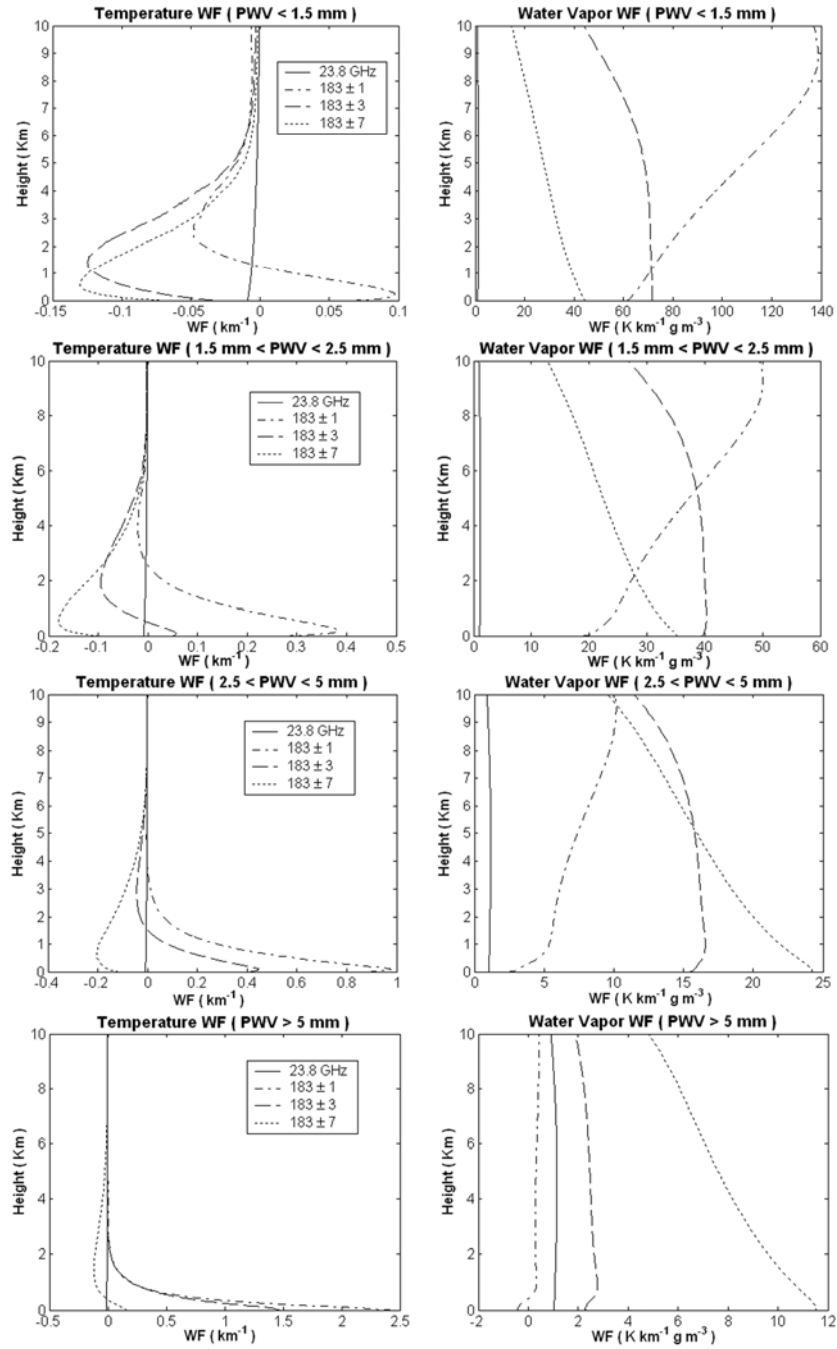
Figure 4 - Average vapor density and temperature weighting functions for four ranges of PWV. The absorption model used is Rosenkranz [5]. After [36].
