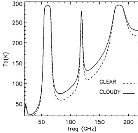
Figure 1 - Calculated brightness temperatures (K) from 20 to 220 GHz for clear and cloudy conditions. The clear calculations are based on a standard atmosphere with the surface values (S) of P_S = 1013 mb, T_S = 293 K, \rho_S = 10 gm -3 , and PWV = 2.34 cm. The cloudy atmosphere contains 1 mm of integrated cloud liquid with a cloud layer of liquid density of 0.1 gm -3 between 1 and 2 km. The absorption models used are given in Figure 2.
