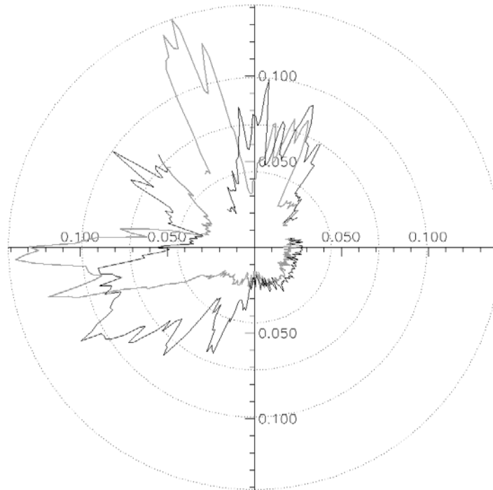
Figure 12 - Series of 14 successive azimuth scans at 30 deg elevation with the multi-channel microwave radiometer MICCY having a beam width of less than 1 deg in all channels. Liquid water path was derived using a regression algorithm employing four frequency channels. After [55].
