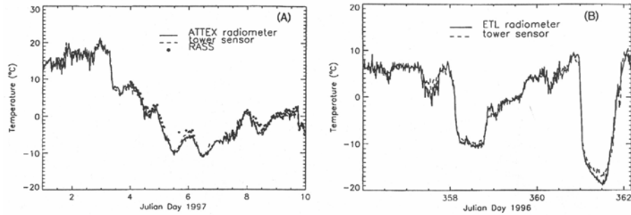
Figure 10 - (A) A 10-day time series of temperature at 200 m as measured by the ATTEX radiometer, by the in situ measurement on the tower, and by a Radio Acoustic Sounding System (RASS). January 1–10, 1997. (B) A 6-day time series of temperature at 200 m as measured by the NOAA radiometer and by the in situ measurement on the tower. December 21–27, 1996. After [54]
