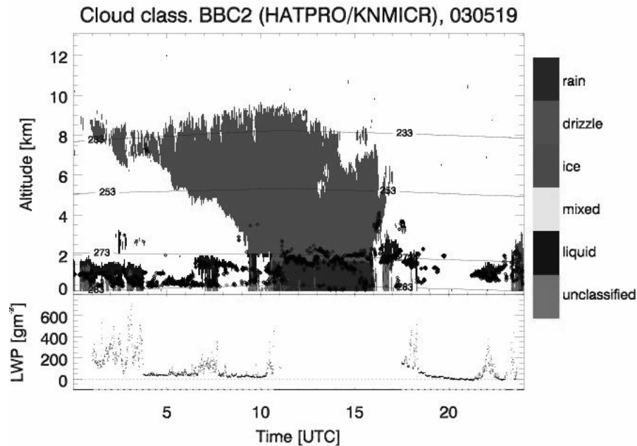
Figure 13 - Cloud classification and LWP for May 19, 2003 at Cabauw. Temperature is derived from interpolated radiosondes. The classification is performed for each individual cloud radar range gate. Black dots indicate the cloud base height as observed by lidar ceilometer.
