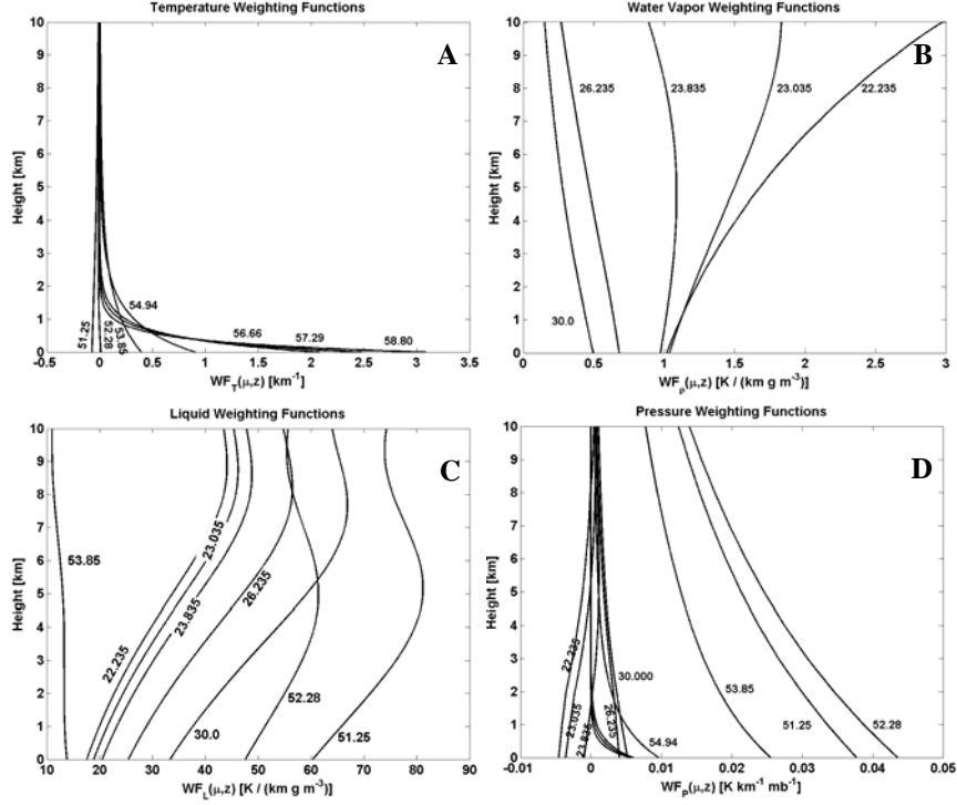
Figure 3 - Weighting functions for the Radiometrics Corporation MWRP. 3A. Temperature weighting functions and center frequencies for V-band channels. High sensitivity to boundary layer temperatures is shown. 3B. Vapor density weighting functions and center frequencies for K-band channels. In conjunction with typical vapor density scale height of approximately 2 km, the vapor density weighting functions provide substantial constraints in the boundary layer. 3C. Liquid density weighting functions for K1-5 and V1-3. The relatively large weighting functions in (a) indicate the K and lower V-band brightness temperature measurements provide significant constraints on the liquid density retrieval. 3D. Pressure weighting functions for all 12-channel. Note that for V1-3, pressure fluctuations are not negligible.
