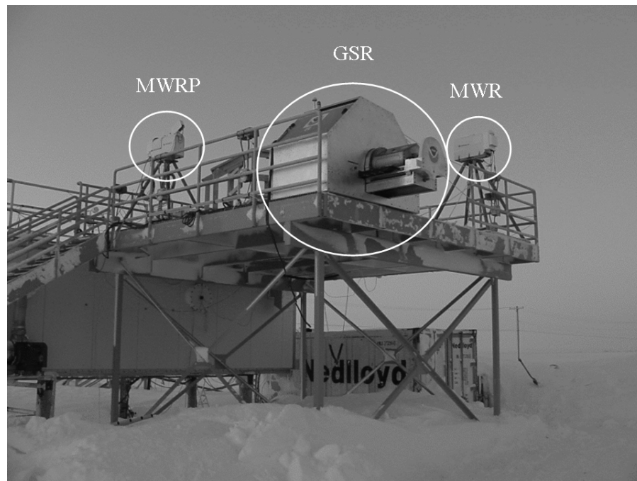
Figure 7 - Photograph of the deployment of the GSR, MWRP, and MWR at the NSA/AO Arctic Winter Radiometric Experiment that was conducted in Barrow, Alaska, USA, during March-April 2004.
