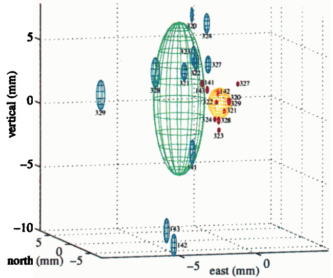
Figure 5. Daily slant (magenta) and zenith (blue) corrected solutions and formal errors using an elevation cut-off of 20 degrees, labeled by day of year. The 11 day, one sigma slant (orange) and zenith (green) corrected solution precisions are also shown. Days 320-329 were observed in 1995, and days 141-143 in 1996.
