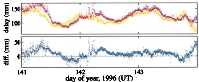
Figure 6. Radiometer sensed slant wet delays at Platteville (magenta) and Table Mountain (orange), projected to zenith, and their difference (blue). We attribute the scatter in each trace to wet delay gradients and the spikes to rain water on the radiometer windows.
