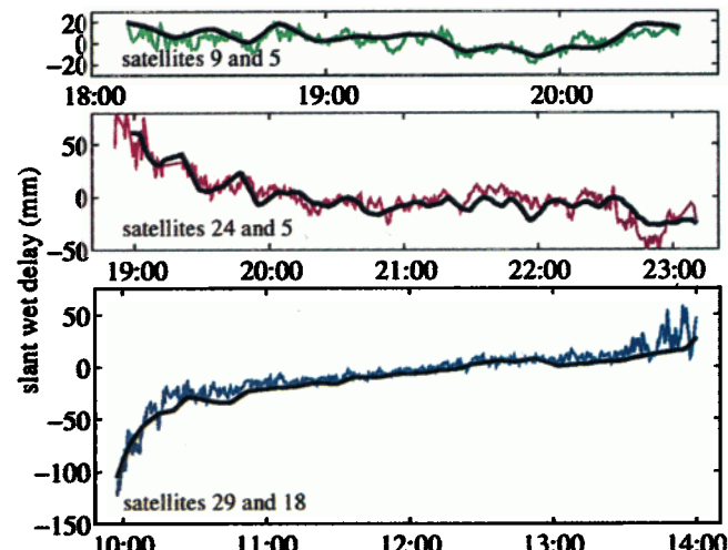
Figure 7. GPS (jagged, color) and radiometer (smooth, black) sensed double difference slant wet delay observations in Universal Time.
