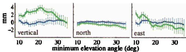
Figure 4. Daily baseline solutions and formal errors for pairs of 35 cm choke ring antennas with (blue) and without collars (green).
